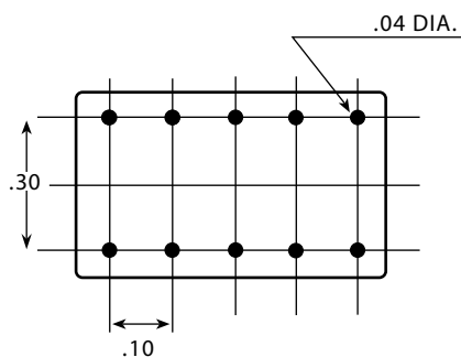
DRILLING PLAN
